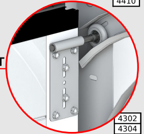
TOP BRACKET
